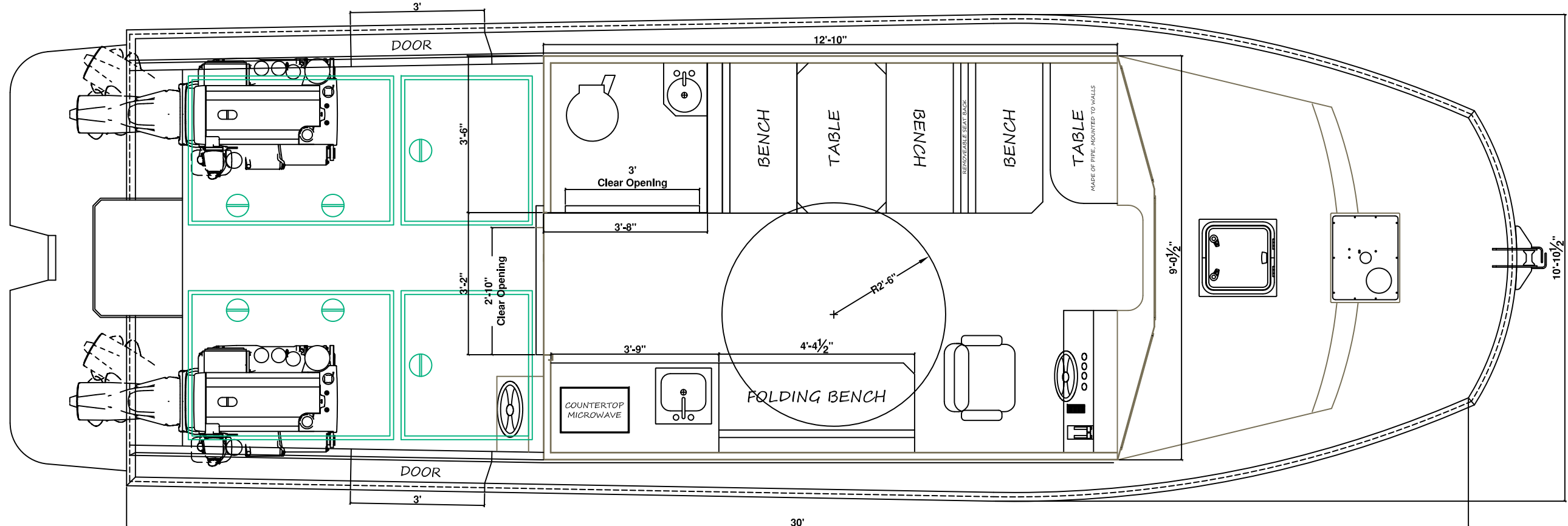
General Arrangements
